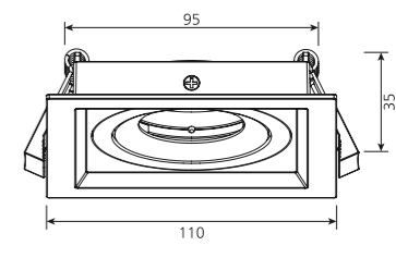
SQUARE TILT TRIM Ø95
