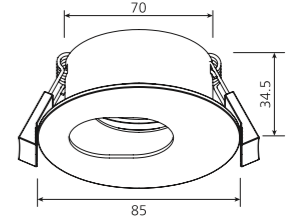
OVAL HOLE TRIM Ø80
