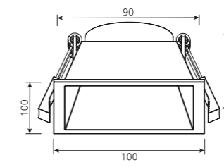
SQUARE DEEP TRIM Ø95
