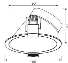
ASYMMETRICAL TRIM Ø95
